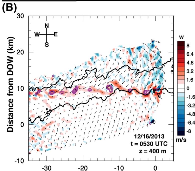
FIG. 4. DOW observations of misocyclones in LLAP lake-effect snowbands. (a) The reflectivity and Doppler velocity of a band observed on 26 Jan 2014 (IOP 20). Black circles indicate locations of misocyclones. (b) Dual-DOW synthesis of misocyclones from a band observed on 16 Dec 2013 (IOP 4). Vectors depict the band-relative horizontal winds, color contours depict vertical motion, black contour is the 20-dBZ isopleth, and magenta contours indicate vertical vorticity (from Kosiba et al. 2016, unpublished manuscript).
