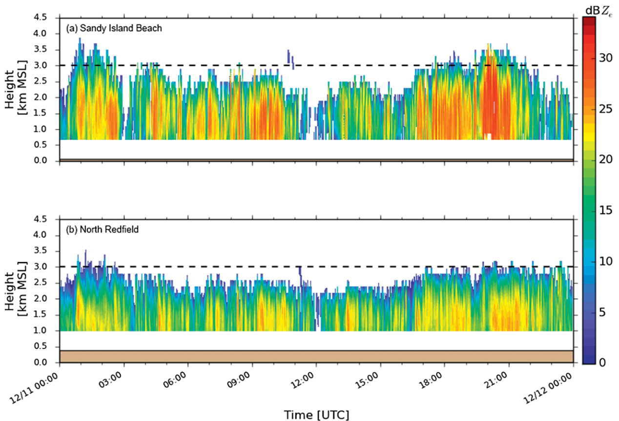
FIG. 2. Time–height plot of the equivalent radar reflectivity factor Z_e measured by MRR profiling radars during IOP 2b at (a) Sandy Island Beach and (b) North Redfield. Heights below ground level at each site are shaded in tan. Data are unavailable in the lowest few 100 m above ground. The dashed black line shows the 3 km MSL height for reference. This figure is adapted from Minder et al. (2015, their Fig. 6).
